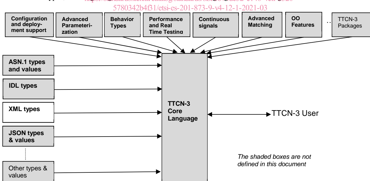
Figure 1: User's view of the core language and its packages
