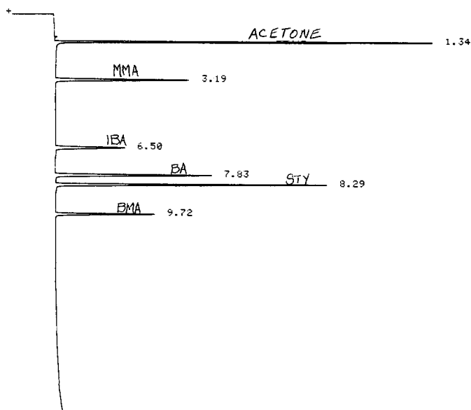
FIG. 1 Typical Chromatogram
