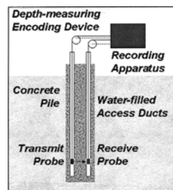
FIG. 3 Test Arrangement
