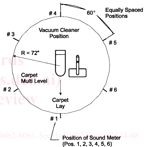
FIG. 3 Sound Test Pattern for Canisters
