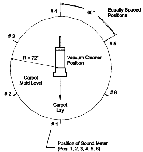
FIG. 2 Sound Test Pattern for Uprights
