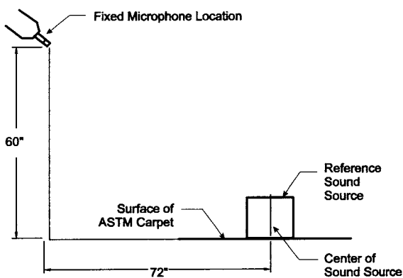
FIG. 1 Sound Set Up
