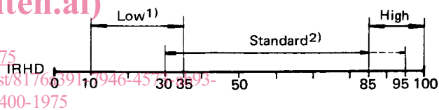
FIGURE 1 – Range of applicability of hardness tests
