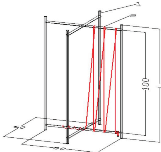
Figure 1 — Winding frame
