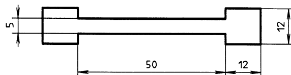
Figure 2 — Dumb-bell test piece
