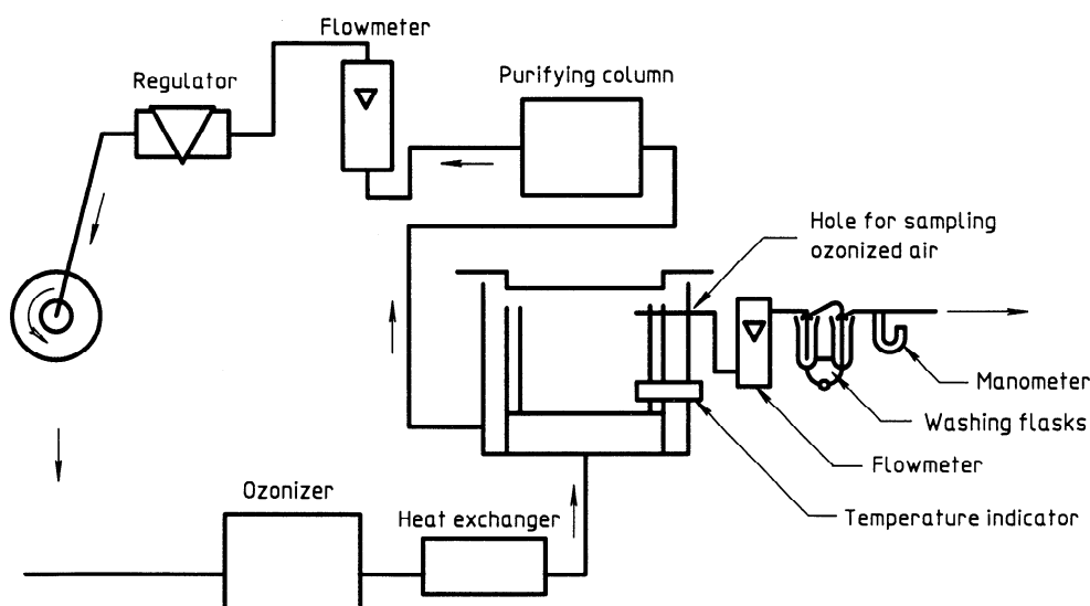
Figure 1 — Schematic diagram of the apparatus
