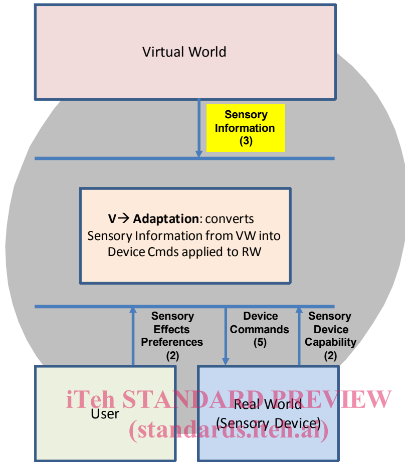
ISO/IEC 23005-3:2013 https://standards.itih.ai/catalog/standards/sist/f46bdc4e-39f4-4a34-b1c9-5c4675c23c8d/iso-iec-23005-3-2013 Figure 1 — System Architecture
