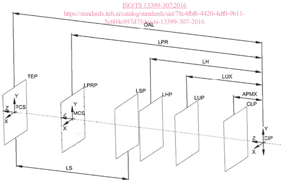
Figure 4 — Planes for design
