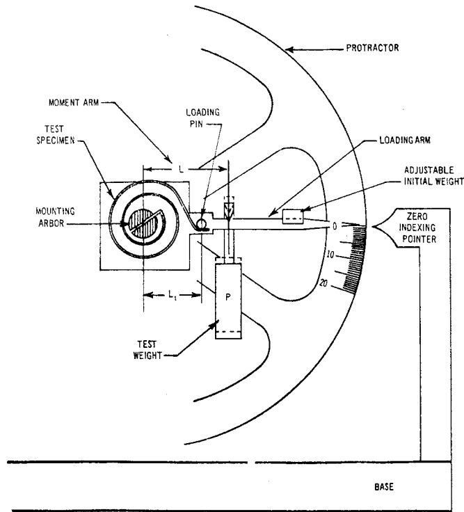
FIG. 1 Schematic Design of Apparatus
