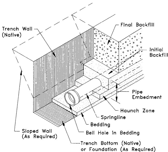
FIG. 1 Installation Terminology
