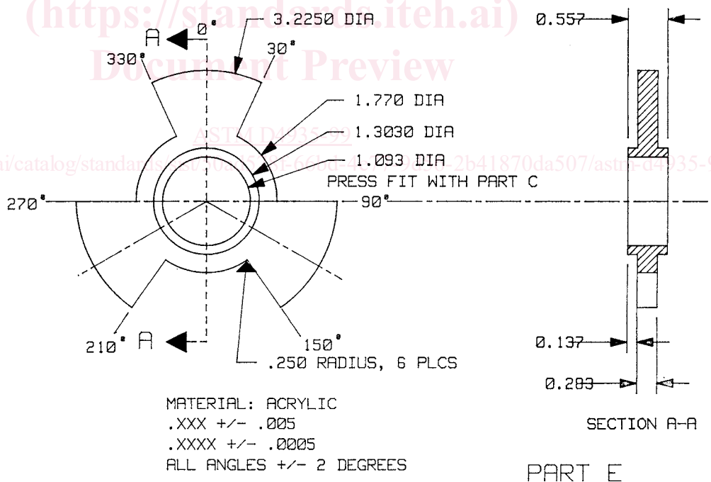
FIG. A1.5 Part E, Support Piece for Center Conductor
