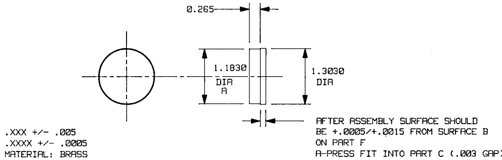
FIG. A1.4 Part D, Pressure Piece for Center Conductor
