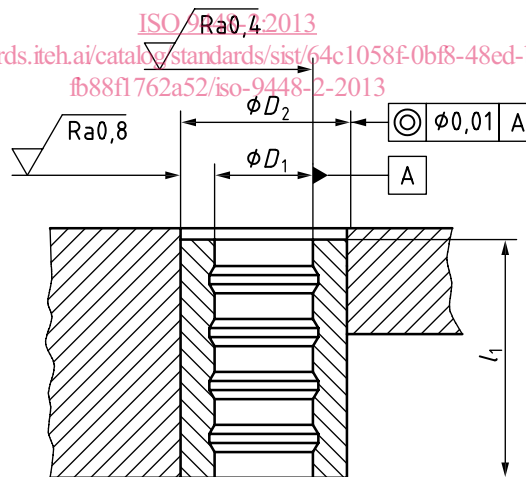
Figure 1 — Form A, plain gliding guide bushes, type 1
