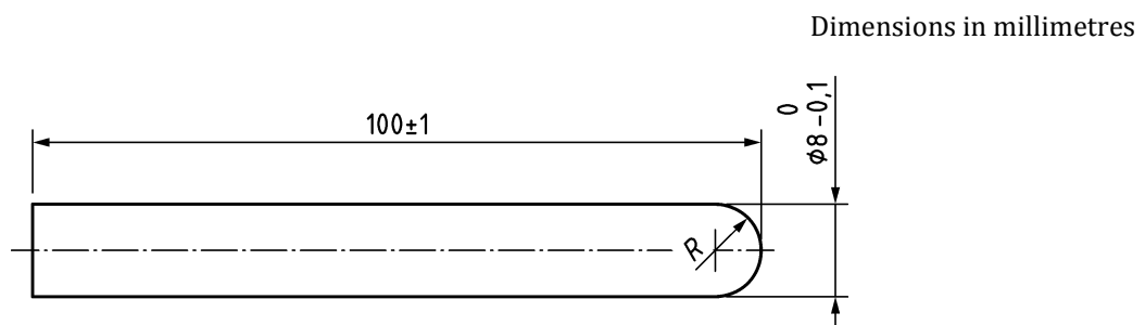
Figure 2 — 8 mm finger rod
