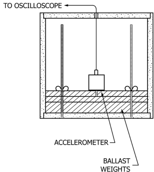
FIG. 2 Test Block
