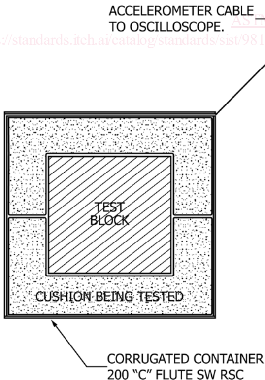
FIG. 1 Specimen Ready For Test
