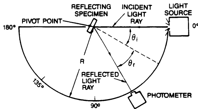
FIG. 1 Apparatus Set-Up
