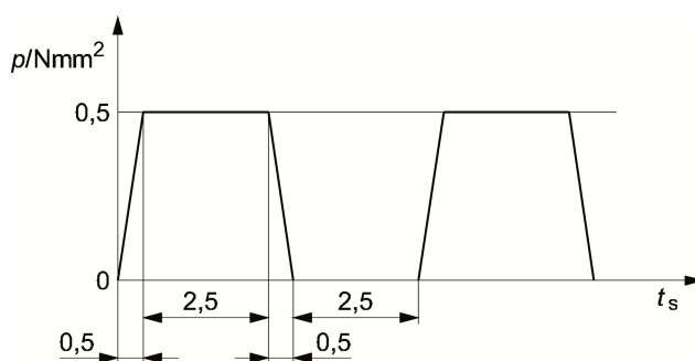
Figure 1 — Dynamic pressure load function
