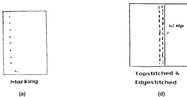
FIG. 9 Lapped Seam for Leather or Nonwoven Fabric from Face Side of Material
