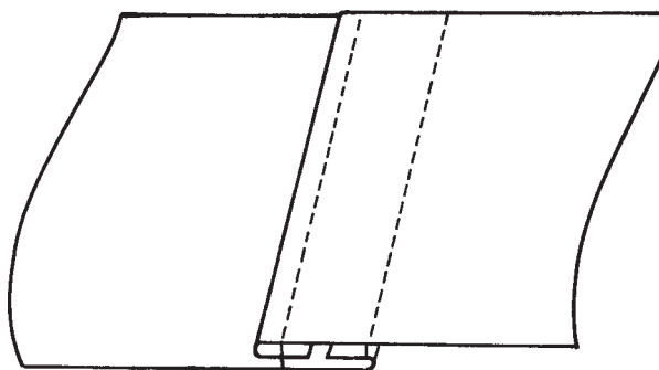
FIG. 5 Flat-Felled Seam from Face Side of Fabric
