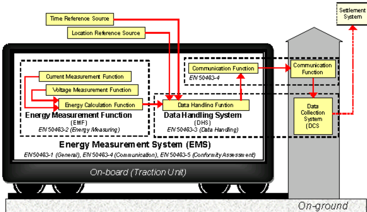
Figure 1 — EMS functional structure and dataflow diagram (standards.iteh.ai)
