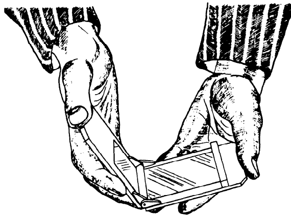
FIGURE 2 – Type 1 bend test apparatus in use
