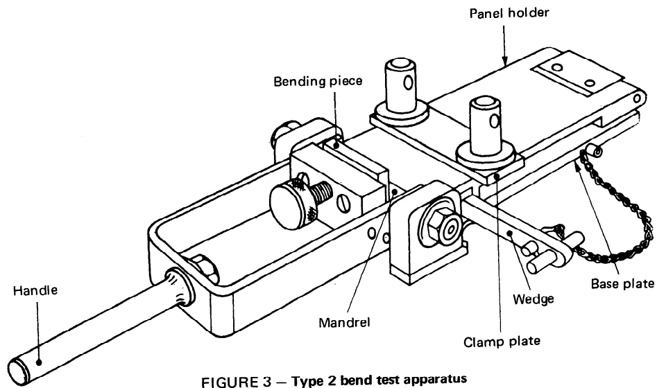
FIGURE 3 – Type 2 bend test apparatus
