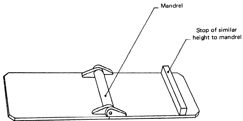
FIGURE 1 – Type 1 bend test apparatus
