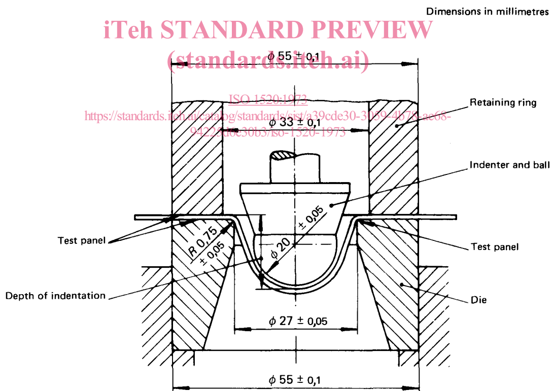
FIGURE – Cupping test apparatus
