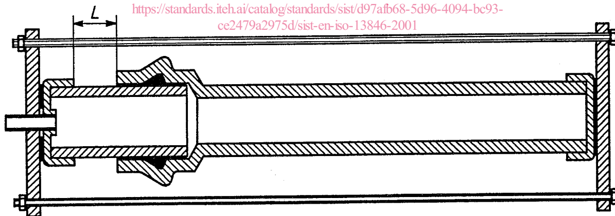
Figure 3 — Example of integral joint type test assembly
