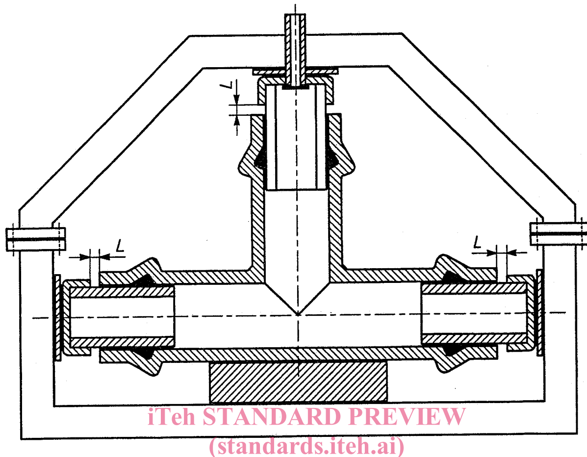
Figure 2 — Example of elastomeric sealing ring type test assembly
