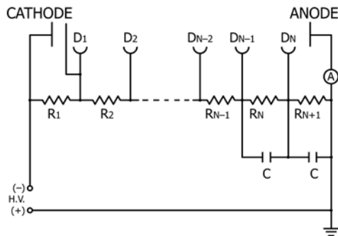
FIG. 4 Voltage-Divider Bridge
