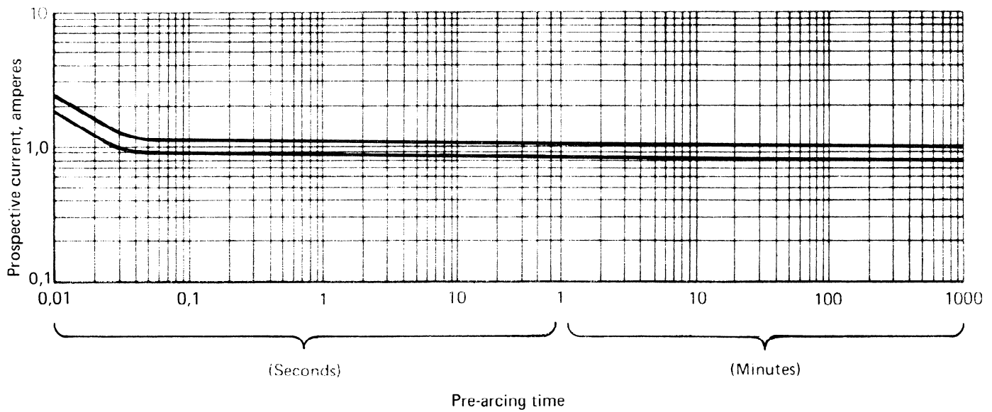
FIGURE 2 – Type B.1; 0,5 A
