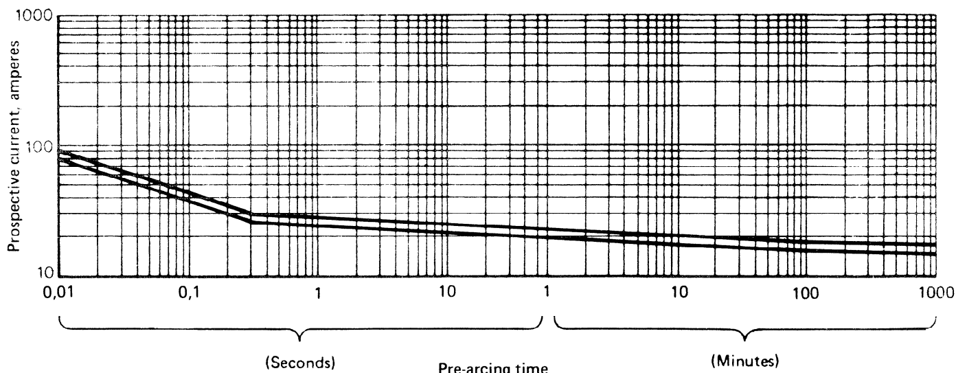
FIGURE 8 – Type B.1; 12,5 A
