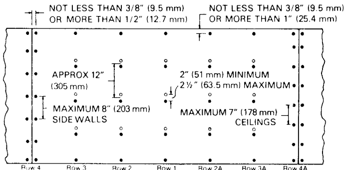
FIG. 3 Double Nailing
