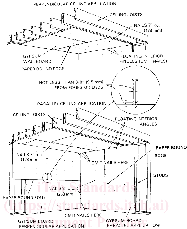
FIG. 2 Single Nailing
