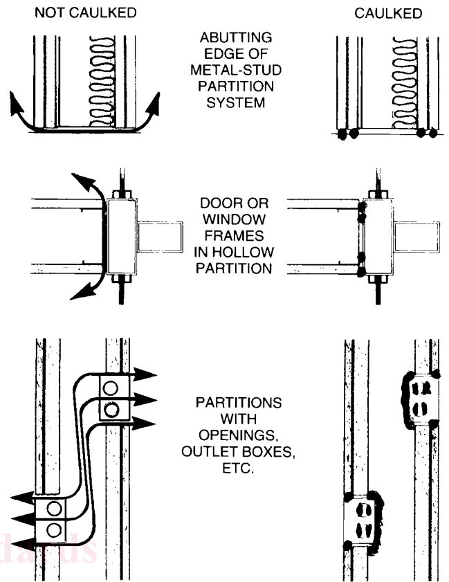
ARROWS SHOW SOUND TRAVEL PATH AROUND OR THROUGH PARTITIONS. FIG. 2 Examples of Achieving an Effective Sound Barrier and Maintaining the Designed STC Value of Partition Systems
