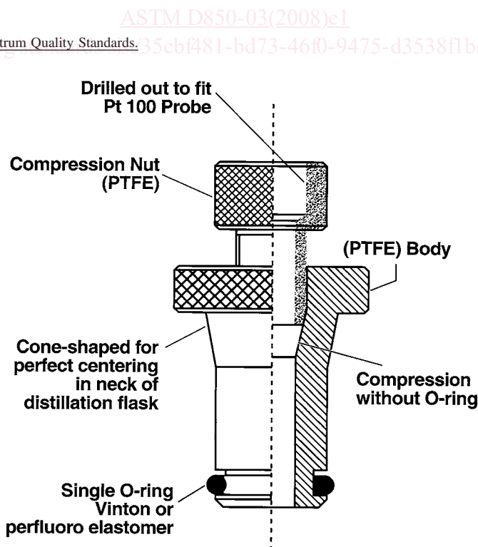
FIG. 2 Examples of Centering Device Designs for Straight-Bore Neck Flasks
