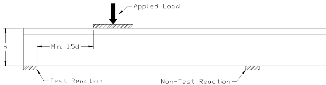
FIG. A1.4 Five-Point Intermediate Reaction Test Set-up
