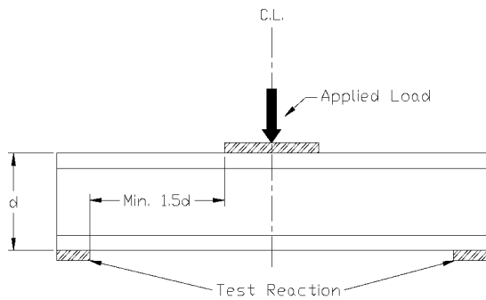
FIG. A1.1 End Reaction Test Set-up (non-symmetric set-up allows for two end-bearing tests per specimen)
