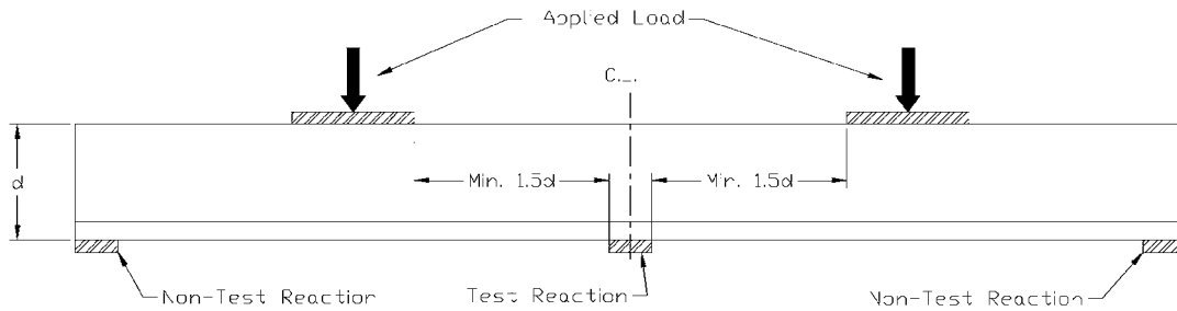
FIG. A1.3 Three-Point Intermediate Reaction Test Set-up
