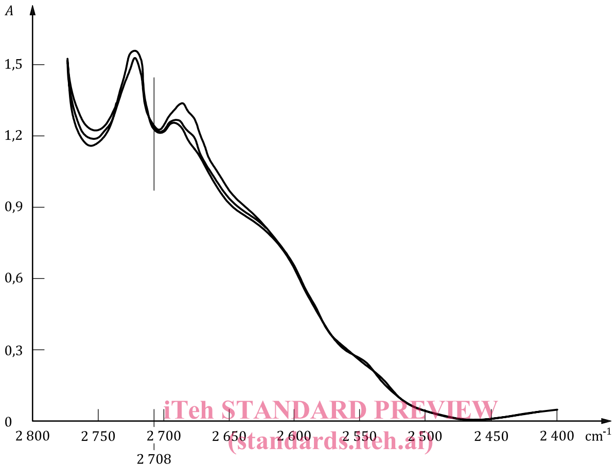
ISO 16565:2013 Figure 2 — FT-IR thickness gauge — Group 1 http://standards.iteh.ai/catalog/standards/sist/23675300-2013-0447-85ff-76200184c6d2/iso-16565-2013
