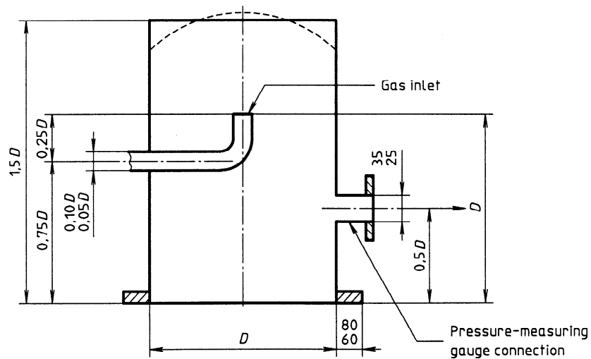
Figure 1 — Test dome
