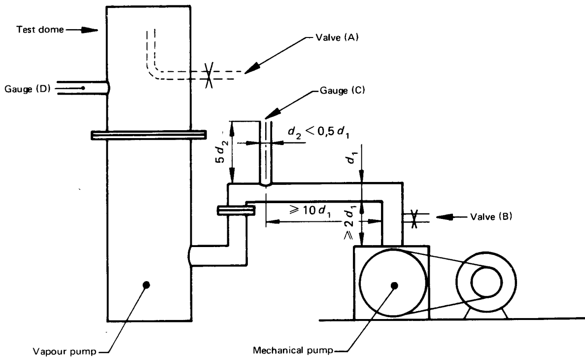
FIGURE 2 – Arrangement of test equipment
