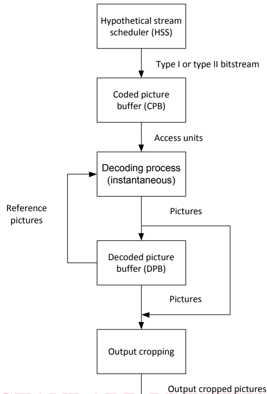
iTeh STANDARD PREVIEW (standards.iteh.ai) Figure C-2 – HRD buffer model
