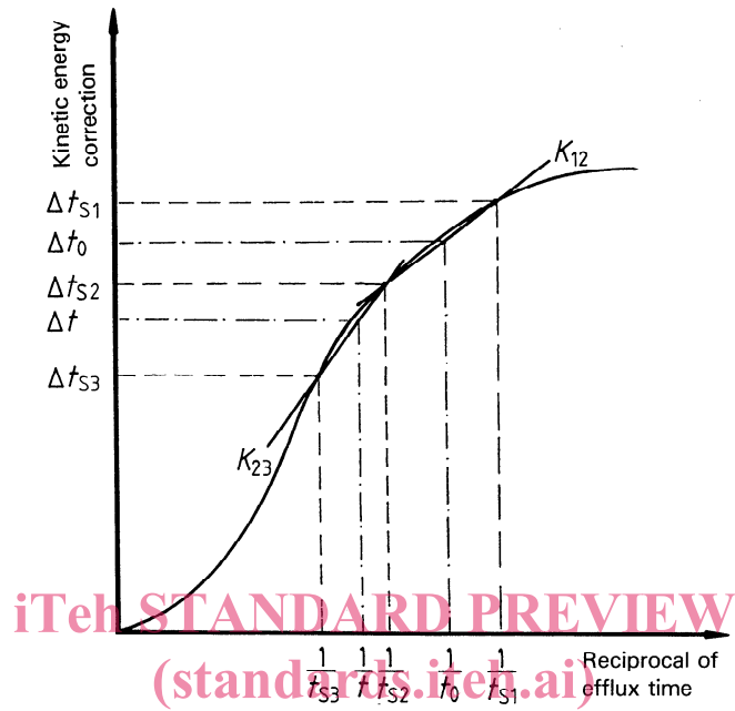
ISO 1628-6:1990 https://standards.iteh.ai/catalog/standards/sist/71874081-1364e86-b0857ab84d6c1011d1c8-6-1990 Figure A.1 — Kinetic energy correction as a function of the reciprocal of efflux time
