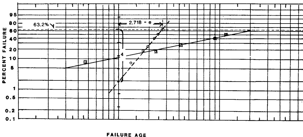
FIG. 1 Representative Weibull Plot Showing the First 5 Failures of a Group Specimen of 9.
