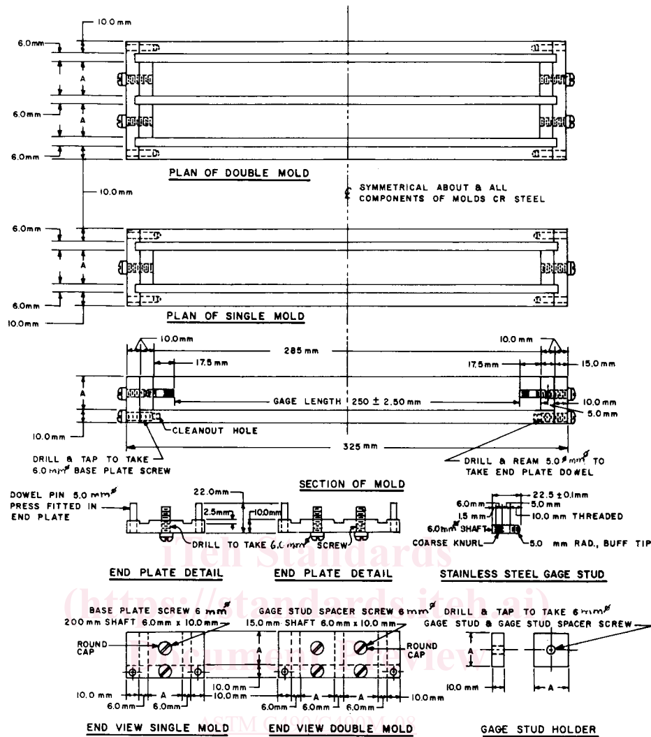
NOTE—Dimension A to be specified by the purchaser. FIG. 1 Molds (SI Units)
