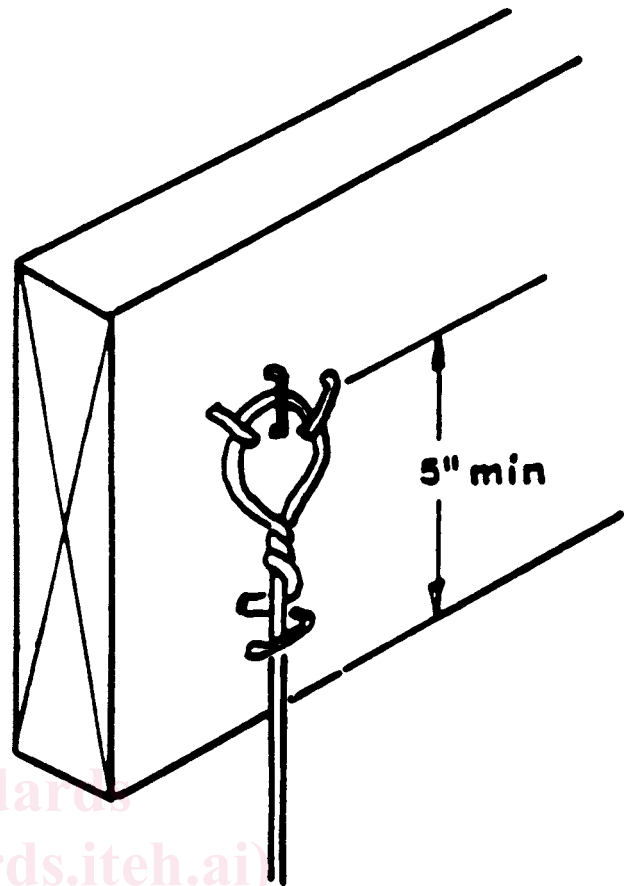
FIG. 3 Hanger Attached to Support Using Staples
