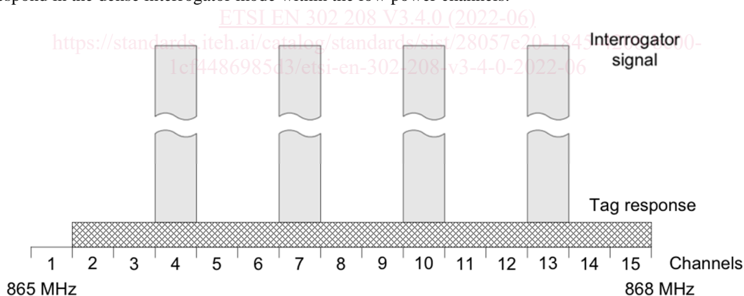
Figure 1: Channel plan for lower band
