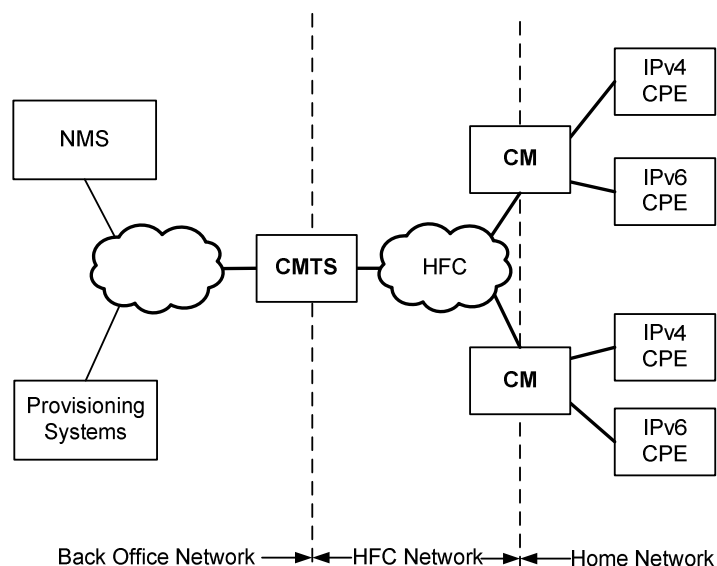
Figure 1: DOCSIS network
