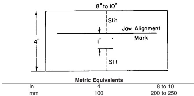
FIG. 2 Illustration of Modified Grab Test Specimens
