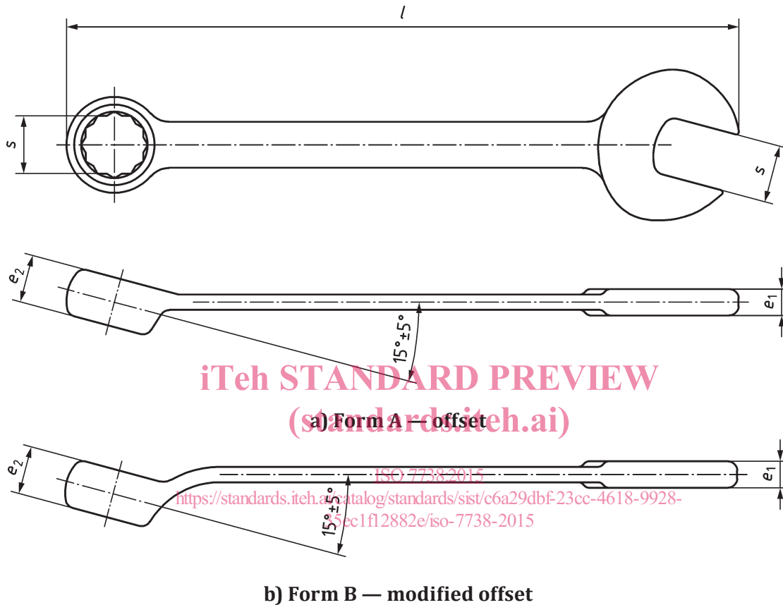
Figure 1 — Combination wrenches
