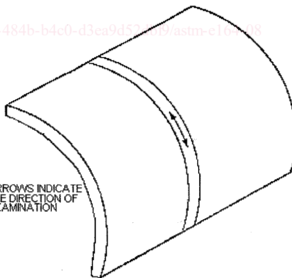
NOTE 1—Search-unit shoes are machined to match the curvature of the work piece when diameter is less than 20 in. (500 mm).
