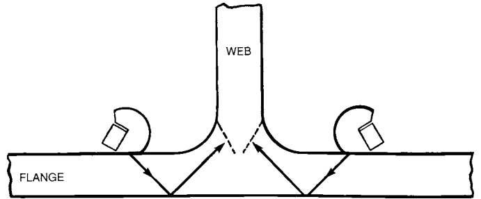
FIG. 8 (b) Alternative Technique 7, for Searching T-Welds for Discontinuities
