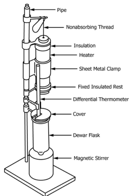
FIG. 1 Specific Heat Calorimeter
