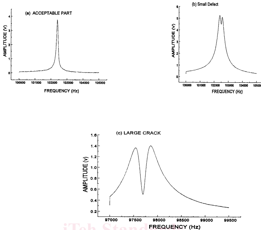
FIG. 3 Shown is a Bending Mode Within a Resonance Spectrum of an Acceptable Steel Cylinder (a), One With a Small Defect (b), and One With a Large Crack (c).
