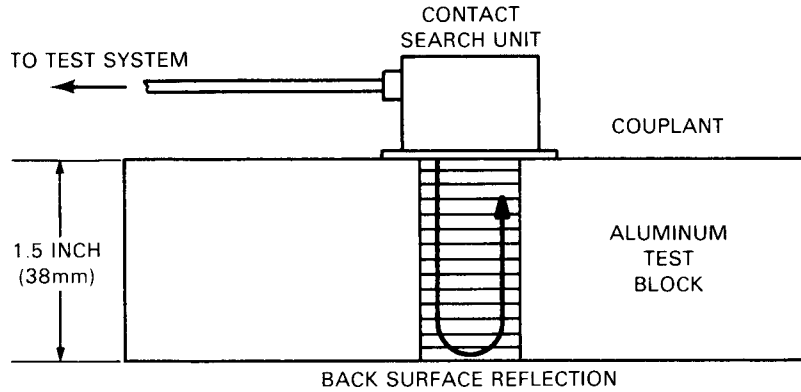
FIG. A1.67 Test Setup for Contact Straight-Beam Search Units
