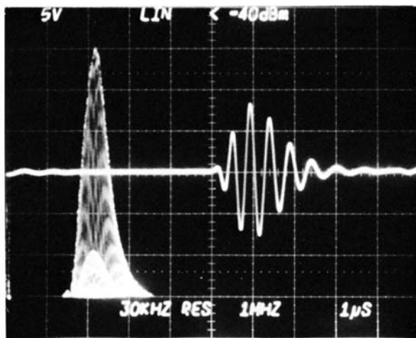
Shock Excitation — Frequency and Time Responses
