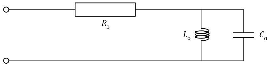
Figure 1 — Excitation-element impedance
