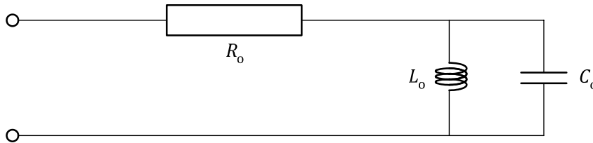
Figure 1 — Excitation-element impedance
