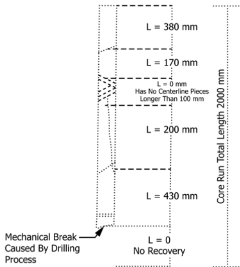
FIG. 1 RQD Logging Center Line Method
