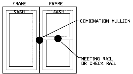
FIG. 3 Combination Mullion with Meeting or Check Rail
