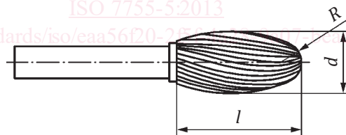
Figure 1 — Hardmetal burr, style E
