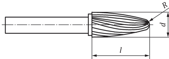
Figure 1 — Hardmetal burr, style F
